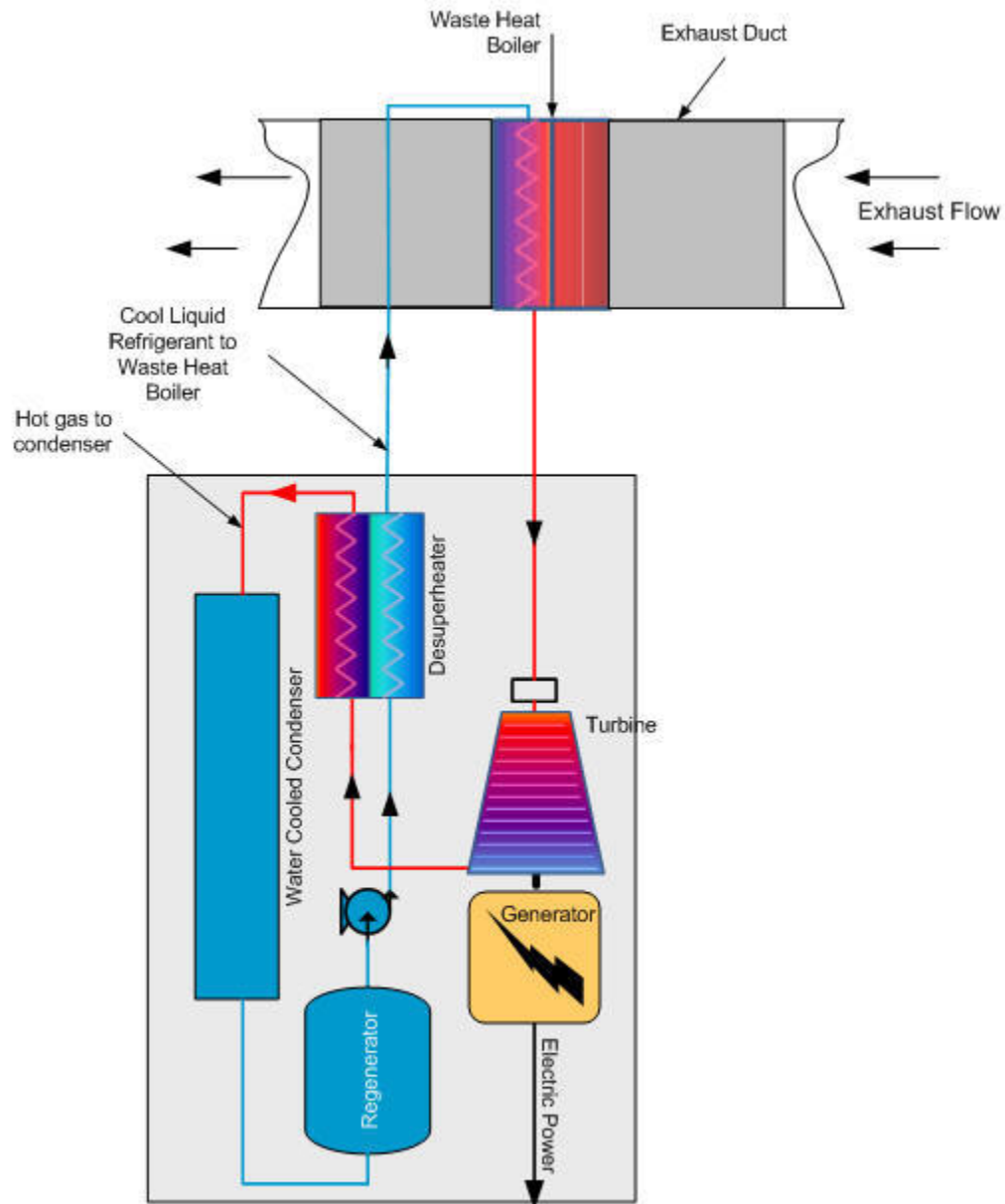
TransPacific Energy flow diagram for heat recovery using flue gas.
